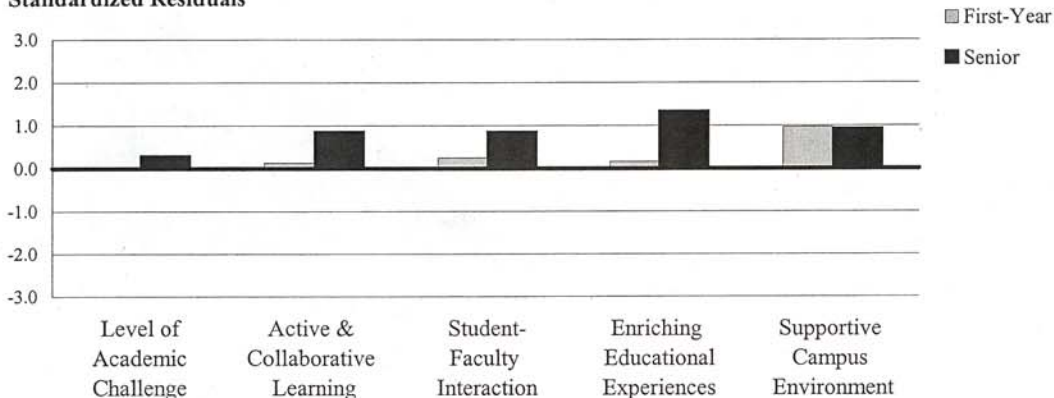
Standardized Residuals
